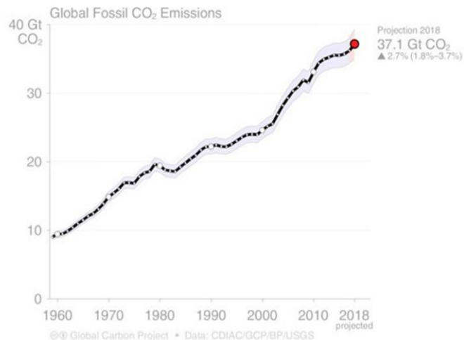
Graph 1. Global fossil CO 2 emissions in the last decades
